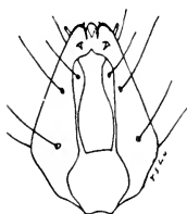
Fig. 554. Ventral aspect of head of Scenopinus fenestralis L.
